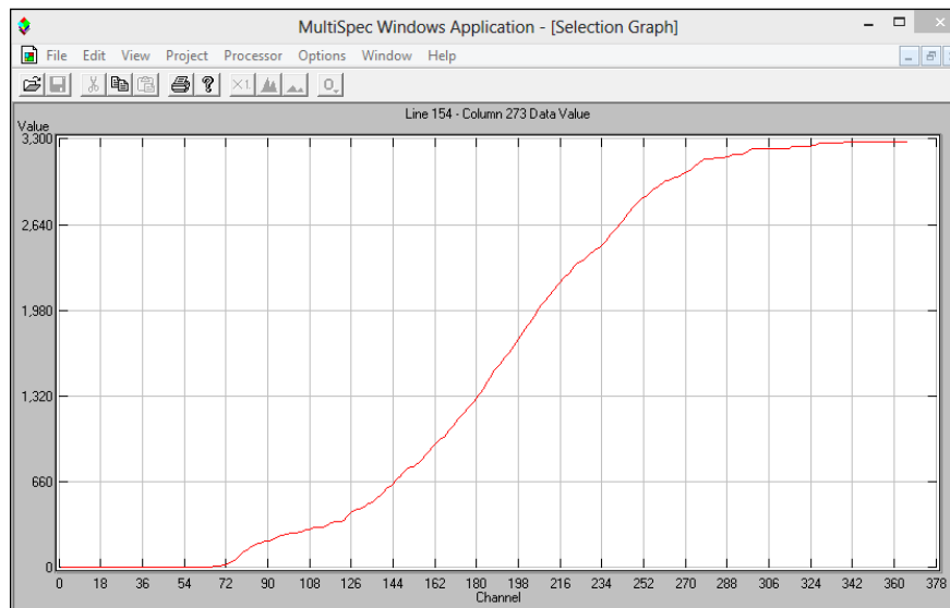
Figure 7. Plot of the accumulated Growing Degree Day vs. day of year
