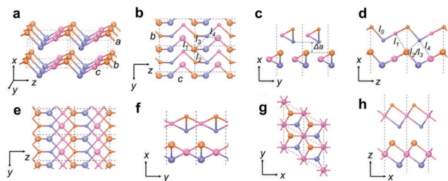
Fig. 4 Structural allotropes for 2D Tellurium. (a–d) Crystal structures of bulk \alpha -Te and bilayer \alpha -Te from the top- (a) and side-views (c and d); (e and f) crystal structures of bilayer \beta -Te from the top- (e) and side-views (f); (g and h) crystal structures of bilayer \gamma -Te from the top- (g) and side-views (h). Reproduced with permission from ref. 16. Copyright 2018, Elsevier.
