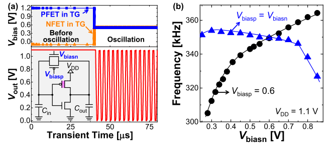
Fig. 3. Single oscillator with FeFET. (a) Pulsing scheme of a single oscillator circuit. (b) f vs. V_{biasn} at V_{biasp} = 0.6 V (circle) and at V_{biasp} = V_{biasn} (triangle).
