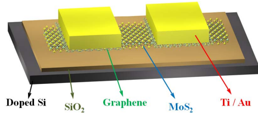
Fig. 1. Structure geometry of hetero-contacts MoS 2 /Graphene/Metal FETs with a channel length of 1 \mu\text{m} .
