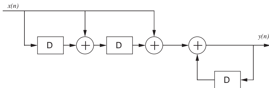
Figure 1: Diagram of a discrete-time system. (D = unit delay)
