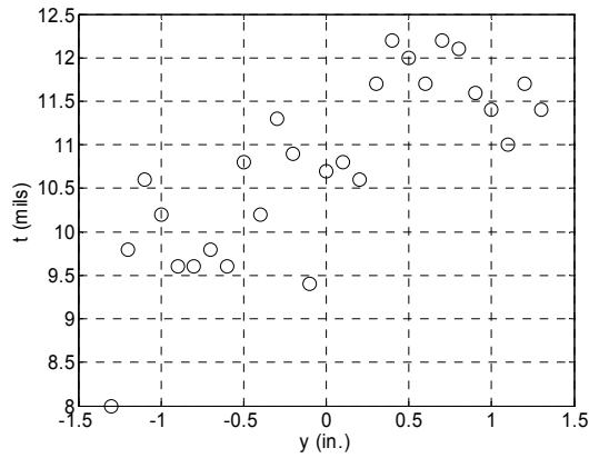
Figure 4. Leading Edge Thickness Variation
