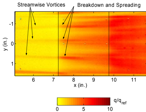
Figure 14. Normalized Heat-Transfer Rate Image with Five 4 mil Thick Roughness Spaced 5/8 inch Apart at 2.57 million/ft Unit Reynolds Number
