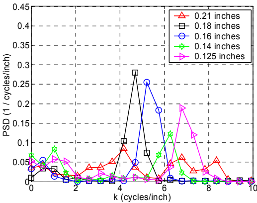
Figure 18. Power Spectral Densities of the Spanwise Heat Transfer Rate Distributions at 8.97 inches from Leading Edge with 2.25 mil Thickness Roughness at 2.72 million/ft Unit Reynolds Number
