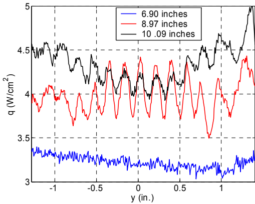
Figure 17. Spanwise Heat Transfer Rate Distributions with 2.25 mil Thick Roughness Spaced 0.16 inches at Unit Reynolds Number of 2.72 million/ft
