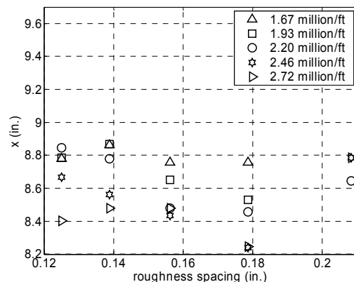
Figure 33. Streamwise Coordinates Corresponding to the Peak Amplitude Ratio with a Roughness Thickness of 2.25 mils
