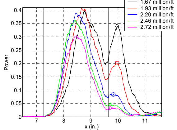
Figure 27. Streamwise Distribution of the Power with 2.25 mil Thick Roughness Spaced 0.16 inches
