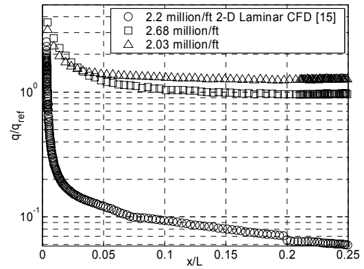
Figure 7. Comparison of Heat-Transfer Rates to CFD Data
