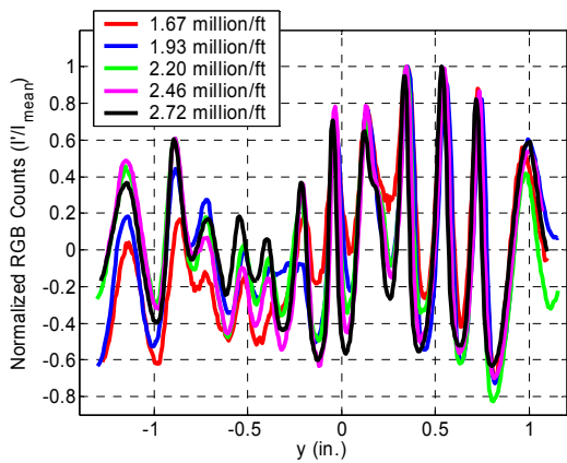
Figure 12. Spanwise Fluctuations Seen in the Oil-Flow Images, at 10.7 inches from the Leading Edge
