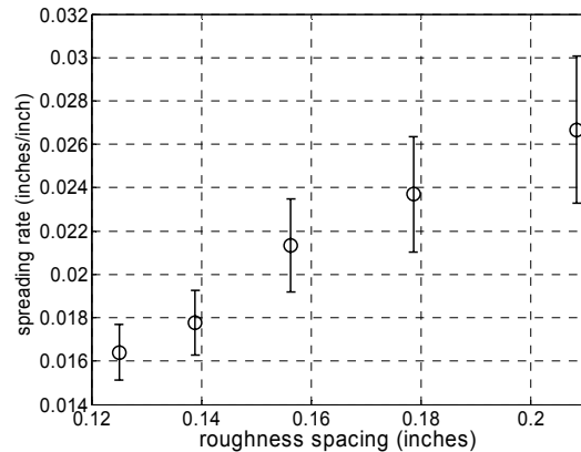
Figure 21. Average Streamwise Vortex Spreading Rate at 8.97 inches from the Leading Edge Using 2.25 mil Thickness Roughness at 2.72 million/ft Unit Reynolds Number
