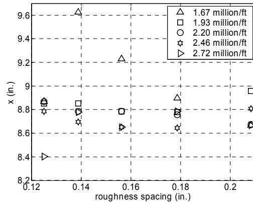
Figure 31. Streamwise Coordinates Corresponding to the Peak Amplitude Ratio with a Roughness Thickness of 1.25 mils
