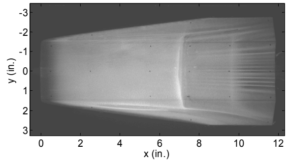
Figure 8. Oil-flow Image for Unit Reynolds number of 2.72 million/ft
