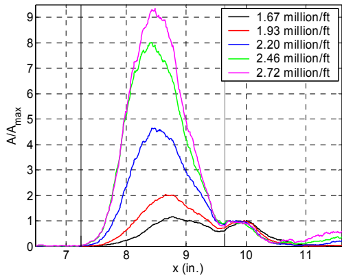
Figure 28. Streamwise Distribution of the Amplification Ratio with 2.25 mil Thick Roughness Spaced 0.16 inches at Several Unit Reynolds Numbers
