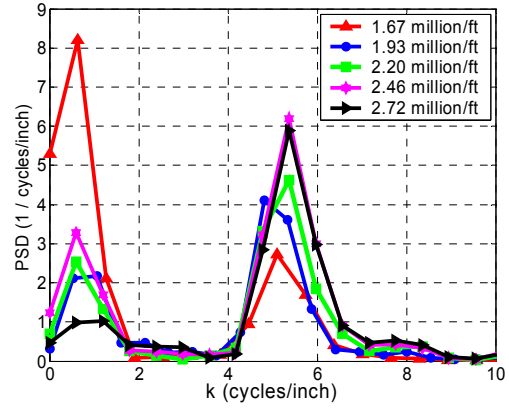
Figure 13. PSD of the Spanwise Fluctuations at 10.7 inches From the Leading Edge
