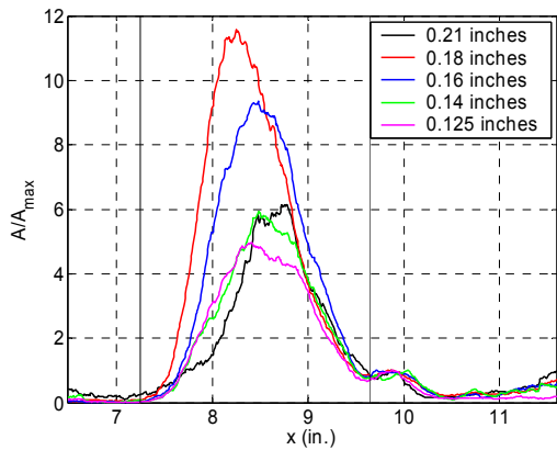
Figure 29. Streamwise Distribution of the Amplification Ratio with 2.25 mil Thick Roughness at 2.72 million/ft Unit Reynolds Number for Several Roughness Spacings
