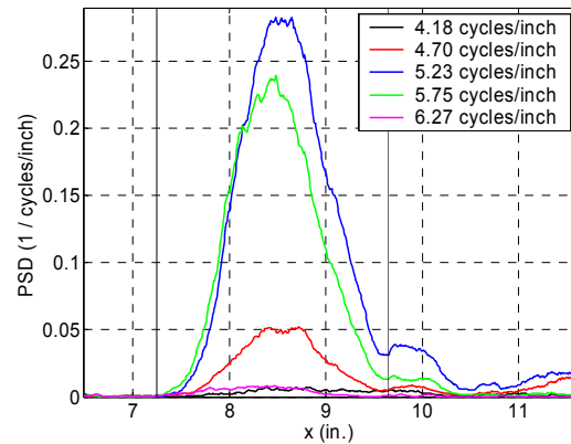
Figure 26. Streamwise Distribution of PSD's Near the Dominant Wave-number with 2.25 mil Thick Roughness Spaced 0.16 inches at Unit Reynolds Number of 2.72 million/ft
