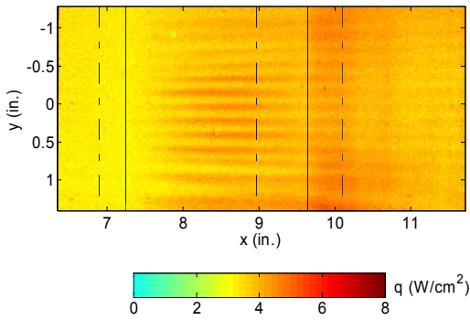
Figure 16. Heat-Transfer Rate Image with 17 Roughness (0.16 inch spacing) of 2.25 mil Thickness at Total Pressure of 127.2 psia (2.67 million/ft.)
