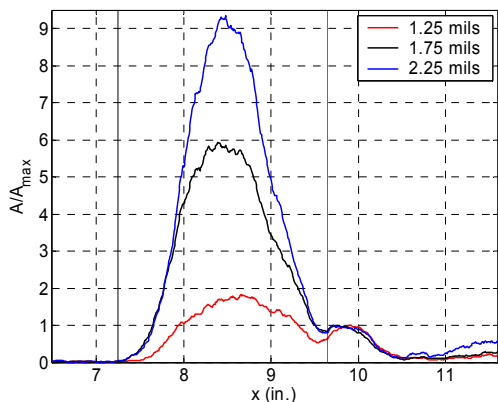
Figure 30. Streamwise Distribution of the Amplification Ratio for with Roughness Spacing of 0.16 inches and Unit Reynolds Number of 2.72 million/ft for Several Roughness Thicknesses
