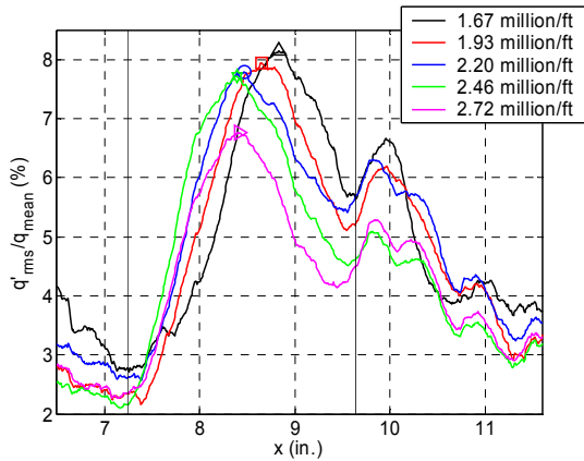
Figure 22. Streamwise Growth of the RMS-Spanwise Heat-Transfer Rate Fluctuations with 2.25 mil Thick Roughness Spaced 0.16 inches
