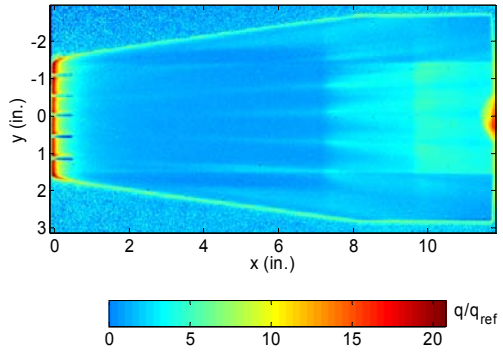
Figure 14. Normalized Heat-Transfer Rate Image with Five 4 mil Thick Roughness Spaced 5/8 inch Apart at 2.57 million/ft Unit Reynolds Number
