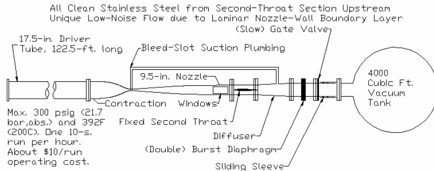
Figure 1. Schematic of the Boeing/AFOSR Mach 6 Quiet Tunnel
