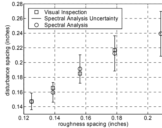
Figure 20. Average Streamwise Vortex Spacing at 8.97 inches from the Leading Edge Using 2.25 mil Thickness Roughness at 2.72 million/ft Unit Reynolds Number
