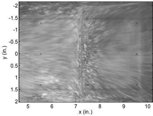
Figure 10. Oil-flow Image with the Oil-Dot Technique at the Lowest Unit Reynolds Number (1.67 million/ft)
