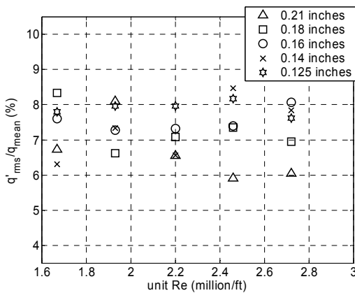
Figure 24. Maximum Normalized RMS Fluctuations on the Second Compression Ramp with Roughness Thickness of 1.75 mils
