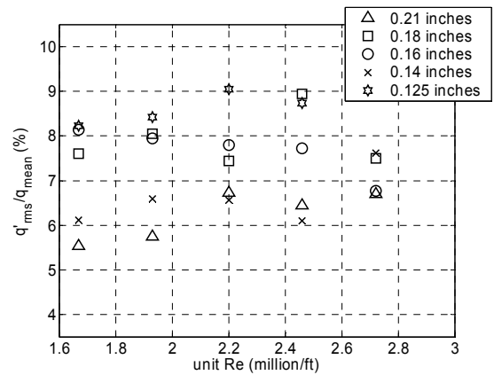
Figure 25. Maximum Normalized RMS Fluctuations on the Second Compression Ramp with Roughness Thickness of 2.25 mils
