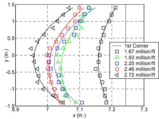
Figure 9. Unit Reynolds Number Effect on the Separation Line
