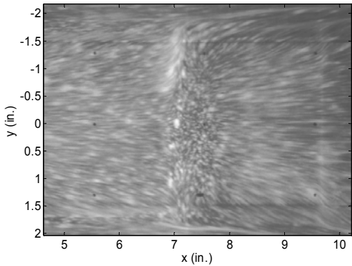
Figure 11. Oil-flow Image with the Oil-Dot Technique at the Highest Unit Reynolds Number (2.72 million/ft)
