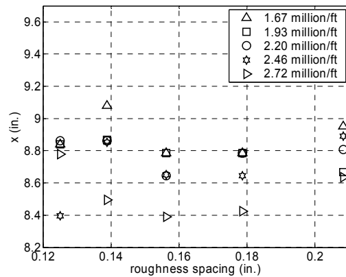
Figure 32. Streamwise Coordinates Corresponding to the Peak Amplitude Ratio with a Roughness Thickness of 1.75 mils
