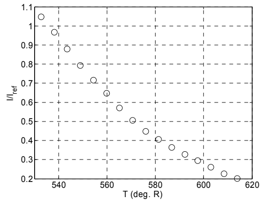
Figure 6. TSP Calibration ( T_{ref} = 536 deg. R.)
