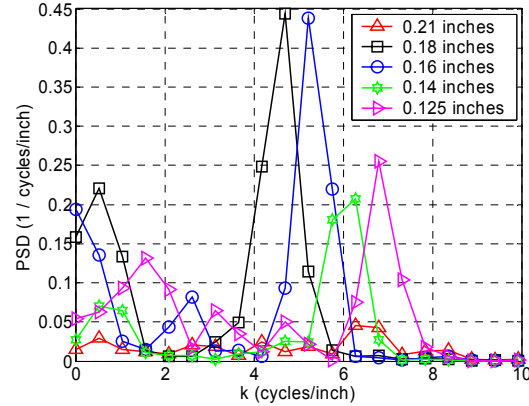
Figure 19. Power Spectral Densities of the Spanwise Heat Transfer Rate Distributions at 8.97 inches from Leading Edge with 2.25 mil Thickness Roughness at 1.67 million/ft Unit Reynolds Number
