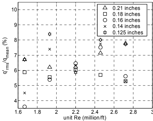
Figure 23. Maximum Normalized RMS Fluctuations on the Second Compression Ramp with Roughness Thickness of 1.25 mils
