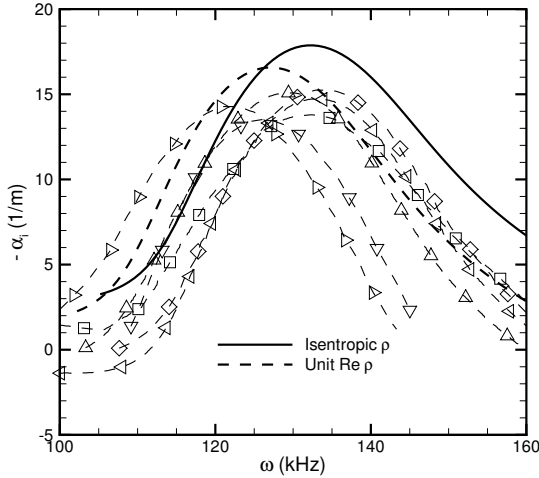
Figure 4: Amplification rates computed using two different values of freestream density for Stetson’s blunt cone at s/r_n = 175 with r_n = 3.81 mm using the conditions given in Table 1. Symbols are defined in Figure 8.
