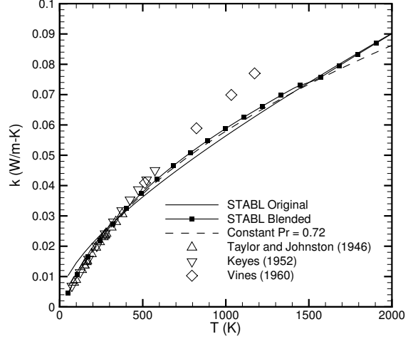
Figure 2: Thermal conductivity as computed by STABL before and after viscosity law modification and with a constant Prandtl number of 0.72 with constant specific heats and the Sutherland law. Experimental data are shown for reference.
