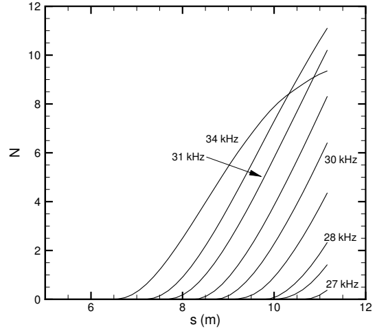
Figure 17: Second mode N factors for the large blunt-ness cone at Mach 8.
