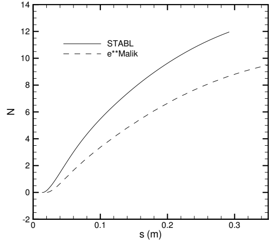
Figure 15: N factors calculated using STABL compared with results of Kimmel [47] using e^{Malik} for a mode at 104 kHz with \beta = 2400 1/m for the sharp cone at Mach 3.5.
