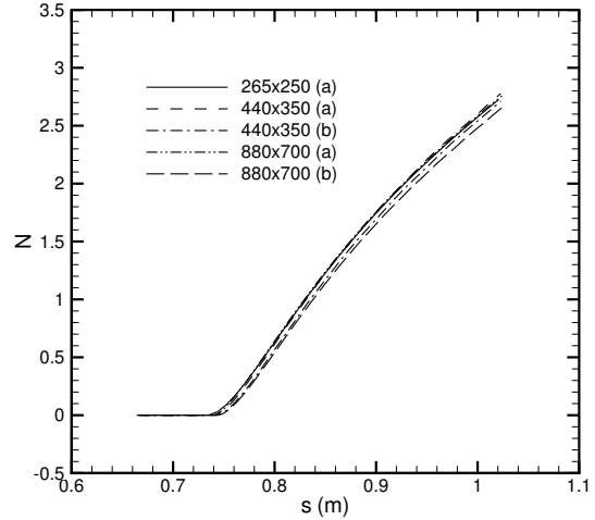
Figure 5: N factors computed using mean flows with varying grid resolutions for Stetson’s blunt cone with r_n = 3.81 mm using the conditions given in Table 1.
