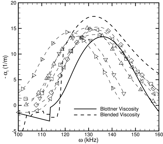
Figure 3: Amplification rate with the original and blended viscosity models for Stetson’s blunt cone at s/r_n = 175 with r_n = 3.81 mm using the conditions given in Table 1. Symbols are defined in Figure 8.
