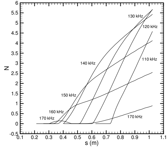
Figure 9: Maximum N factors obtained for various frequencies for the Stetson et al. blunt cone case with r_n = 3.81 mm.
