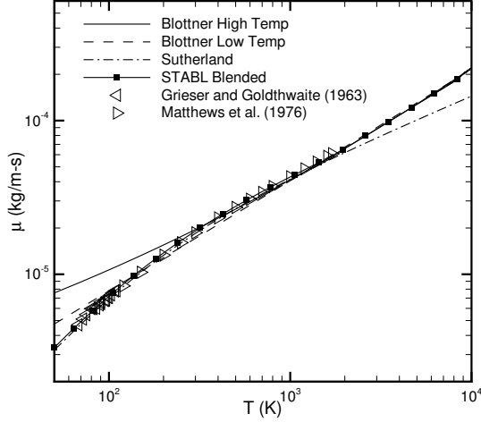
Figure 1: A comparison of the viscosity computed with both sets of coefficients of the Blottner form, the Sutherland law, and experimental data. The line labeled STABL Blended represents the modified method implemented as a result of the author's analysis.
