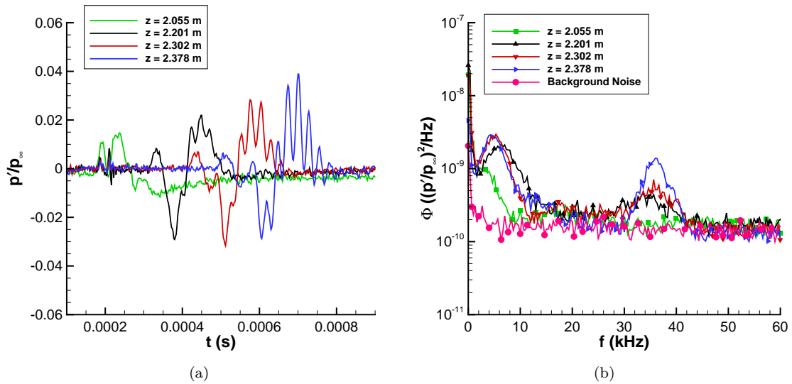
Figure 15. Centerline disturbance measurements at Re = 6.40 \times 10^6/m (a) Time traces; (b) Power-spectral density.
