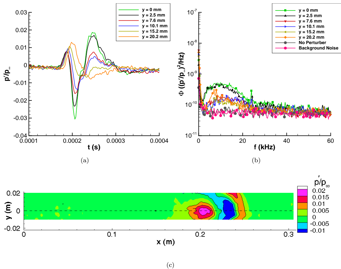
Figure 9. Upstream disturbance measurements at Re = 10.8 \times 10^6/m , z = 2.055 m (a) Time traces; (b) Power-spectral density; (c) Contour plot.
