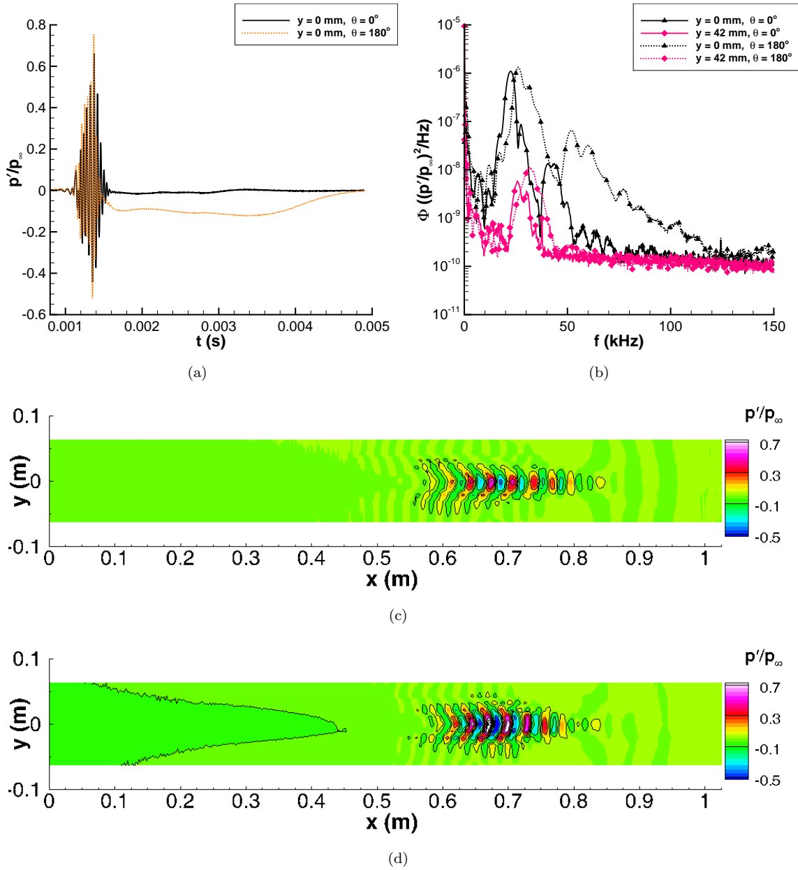
Figure 20. Comparison of disturbances on top and bottom wall of the tunnel at z = 2.781 m, Re = 6.40 \times 10^6 / m (a) Centerline time traces; (b) Power-spectral density; (c) Contour plot on top wall; (d) Contour plot on bottom wall.
