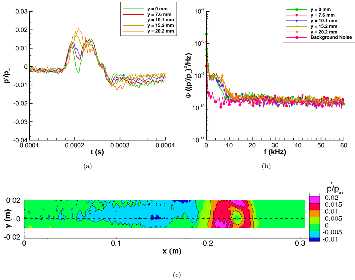
Figure 14. Upstream disturbance measurements at Re = 6.40 \times 10^6/m , z = 2.055 m (a) Time traces; (b) Power-spectral density; (c) Contour plot.
