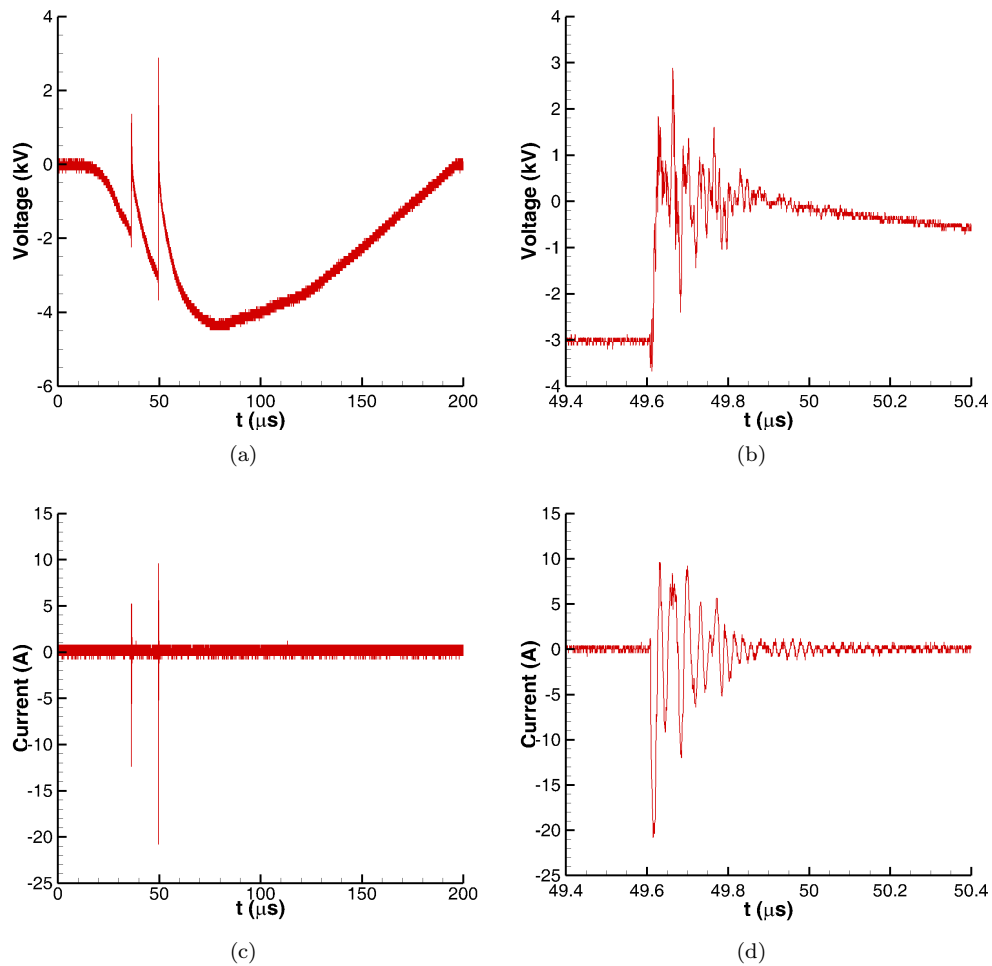
Figure 7. Perturbation measurements showing intermittent sparks superimposed on a glow perturbation, Re = 5.60 \times 10^6/m (a) Voltage; (b) Voltage (detail of second spark); (c) Current; (d) Current (detail of second spark).
