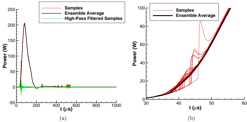
Figure 6. Power measurements showing high-frequency component of perturbation, Re = 6.40 \times 10^6/m (a) Individual samples and ensemble averages; (b) Detail view of high-frequency spikes superimposed on the lower-frequency glow pulse.
