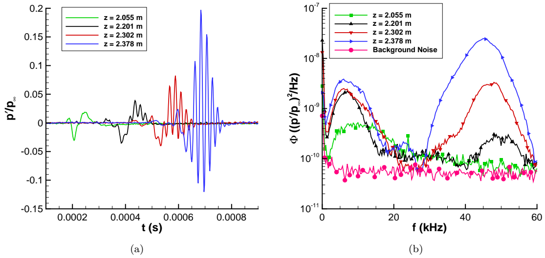
Figure 10. Centerline disturbance measurements at Re = 10.8 \times 10^6/m (a) Time traces; (b) Power-spectral density.
