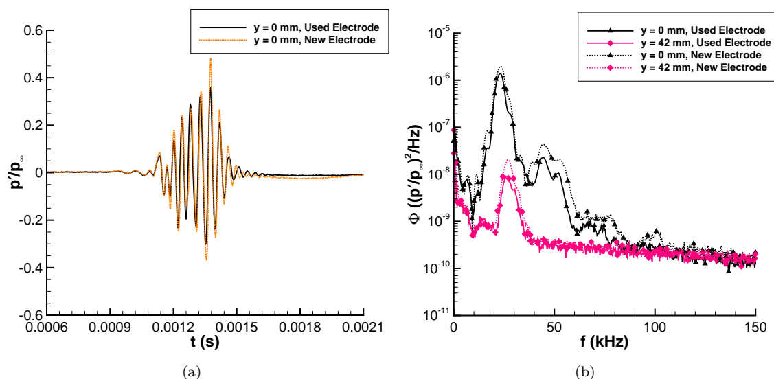
Figure 16. Comparison of disturbances at z = 2.781 m with new and used electrodes, Re = 6.40 \times 10^6/m (a) Centerline time traces; (b) Power-spectral density.
