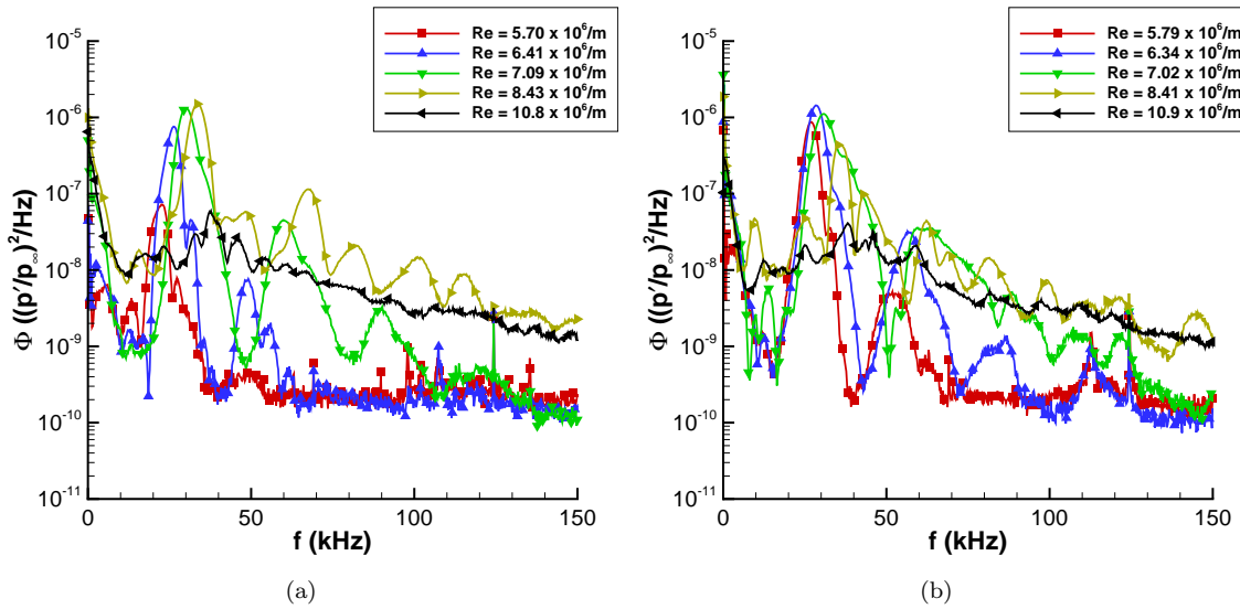
Figure 22. Comparison of centerline disturbances on top and bottom wall of the tunnel at z = 2.730 m (a) Power-spectral density on top wall; (b) Power-spectral density on bottom wall.
