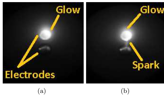
Figure 8. Black and white pictures of perturbation on a cone model, Re = 2.51 \times 10^6/m , P_0 = 255 \text{ kPa} , T_0 = 427 \text{ K} (a) Glow pulse; (b) Combined spark and glow pulse.
