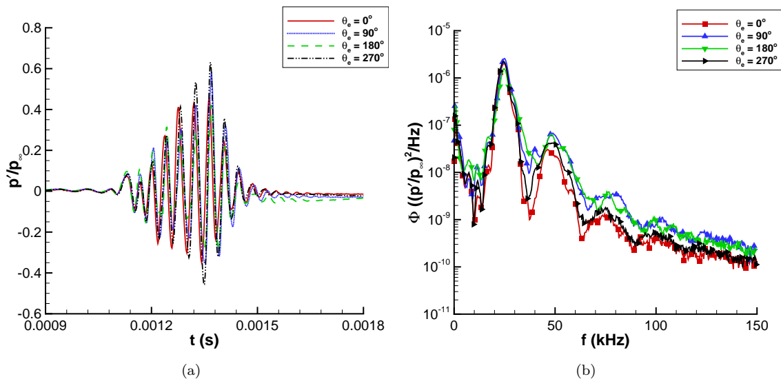
Figure 17. Comparison of centerline disturbances at z = 2.781 m and y = 0 mm with electrode polarity switches and electrode rotation at Re = 6.40 \times 10^6/\text{m} (a) Time traces; (b) Power-spectral density.
