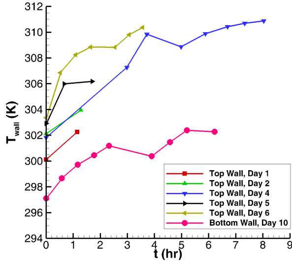
Figure 23. Increase in average wall temperature at z = 2.755 m throughout a testing day, each point corresponds to a measurement before a tunnel run.
