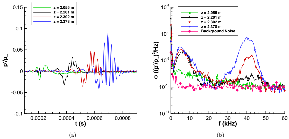
Figure 13. Centerline disturbance measurements at Re = 8.40 \times 10^6/m (a) Time traces; (b) Power-spectral density.
