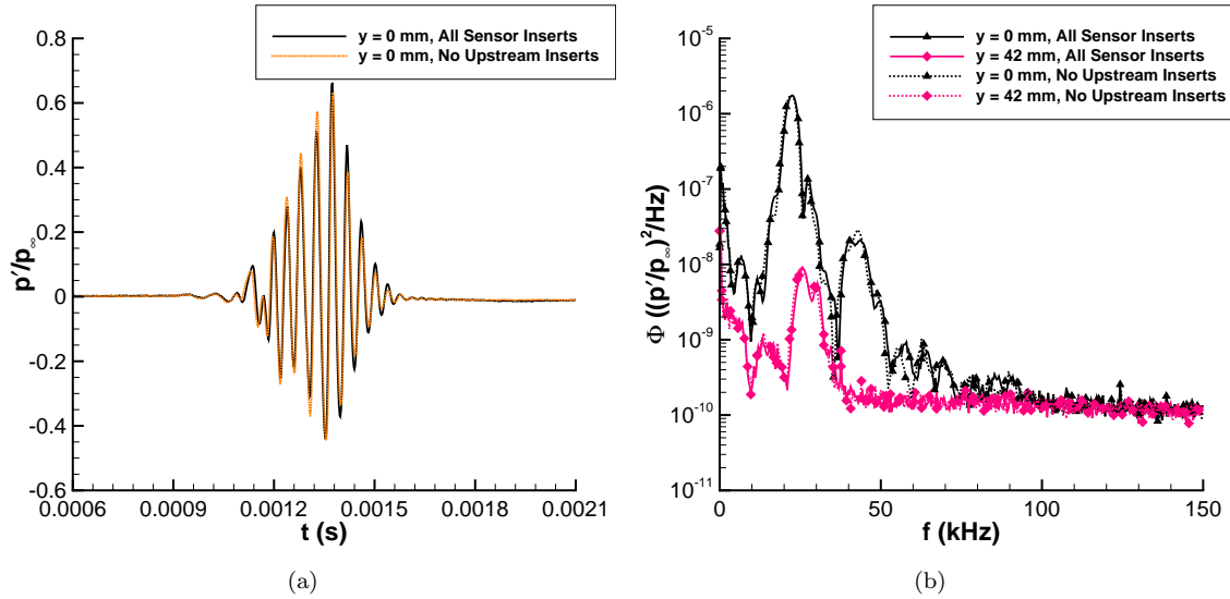
Figure 19. Comparison of disturbances at z = 2.781 m with and without upstream sensor inserts, Re = 6.40 \times 10^6/\text{m} (a) Time traces; (b) Power-spectral density.
