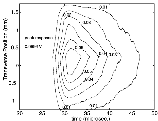
Fig. 6 Contours of constant response for the transverse survey 0.3 s after flow initiation; P_d \approx 65.5 kPa.
