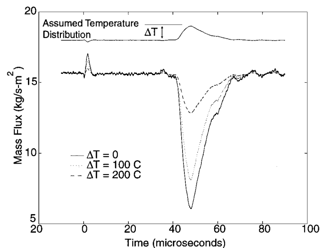
Fig. 7 Calculated mass flux near the thermal spot center 0.3 s after flow initiation.
