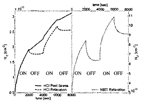
Figure 3: Stress and passivation cycles during the ON and OFF states of AC bias. The model predicts relaxation for HCl degradation. Post-stress trap generation reported in the literature can also be simulated.
