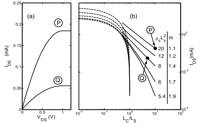
Fig. 5: (a) The source-drain current vs. V_{DS} for V_G - V_{TH} = 1.0 V for two networks P and Q with different densities and L_C (as shown in b) here, L_S = 1 \mu\text{m} and L_W = 200 \mu\text{m} . (b) The on-current vs. normalized channel length computed by analytical model for L_C < L_S (Eq. 4, dotted curves) and numerical model (Eq. 6, solid lines) for V_G - V_{TH} = 1.0 V and V_D = 1 V.
