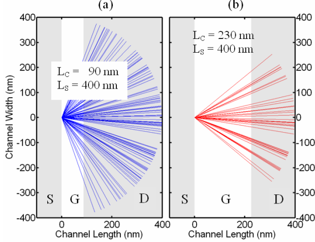
Fig. 2 Fan Diagram : If all sticks in Fig. 1a were collected at a point (with angles preserved), it is easy to see that more sticks connect S/D for a transistor with a shorter channel length. Here, stick length is L_S = 400 nm and channel lengths are (a) L_C = 90 nm and (b) L_C = 230 nm.
