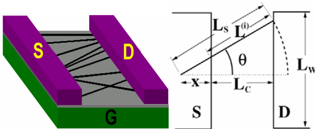
Fig. 1 Geometry of nanobundle network transistor: (a) A schematic of NBT. (b) A nano-stick between the S/D electrodes making an angle \theta with the channel axis.
