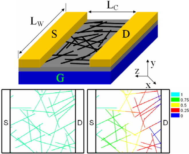
Fig. 4. (a) A schematic of NBT: Geometry of nanobundle network transistor. Distribution of normalized conductance along the sticks in the random network in (b) low and (c) high bias, respectively. The conductance is uniform along the channel in low bias while it varies nonlinearly in the high bias condition resulting in an inhomogeneous percolating network and the contours of conductance are not straight lines parallel to S/D as in conventional MOSFET.
