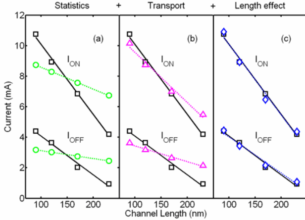
Fig. 3 Experimental [1] (squares with solid line fit) and theoretical (dotted line fits) I_{ON} and I_{OFF} vs. L_C . The inverse scaling of I_{ON} and I_{OFF} with L_C is a consequence of sequential addition of (a) Statistical effect : Increased probability of sticks to bridge S/D as channel length decreases (Fig 2), (b) Transport effect : Prevalence of ballistic transport in shorter channel devices, and (c) Average length effect : Average length for m-SWCNT \langle L_M \rangle \sim 350 nm is made less than s-SWCNTs \langle L_S \rangle \sim 1000 nm. Here, mean free path for s-SWCNT \lambda_D \sim 200 nm. Note that theory matches well with experiment only after all three effects are included in the simulation as shown in (c).
