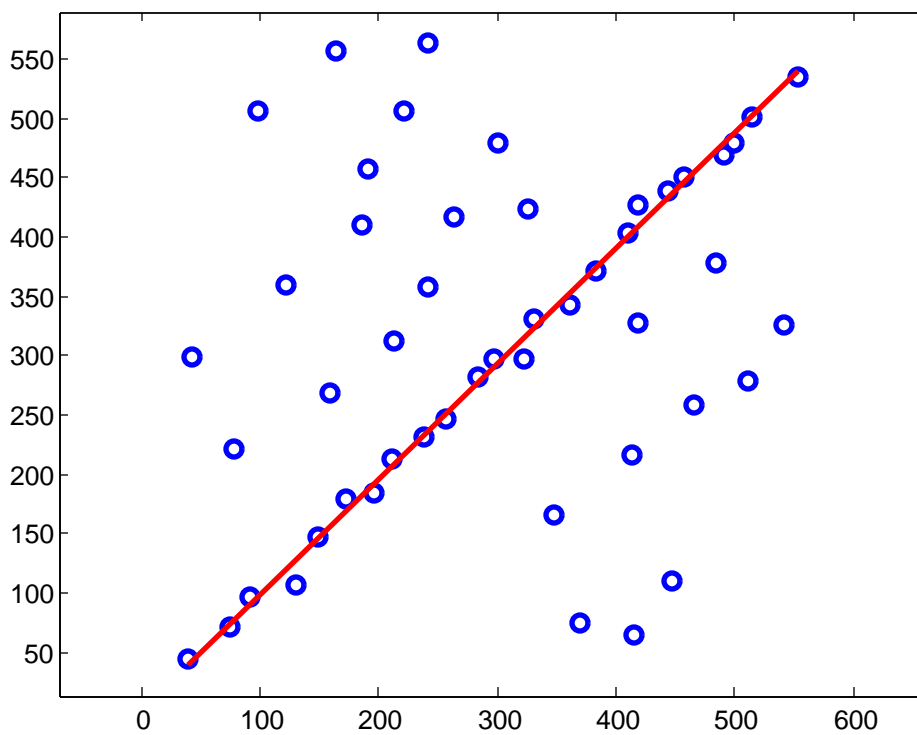
RANSAC fit with max INLIERS
