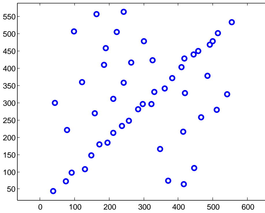
points to consider for LS vs. RANSAC line fit
