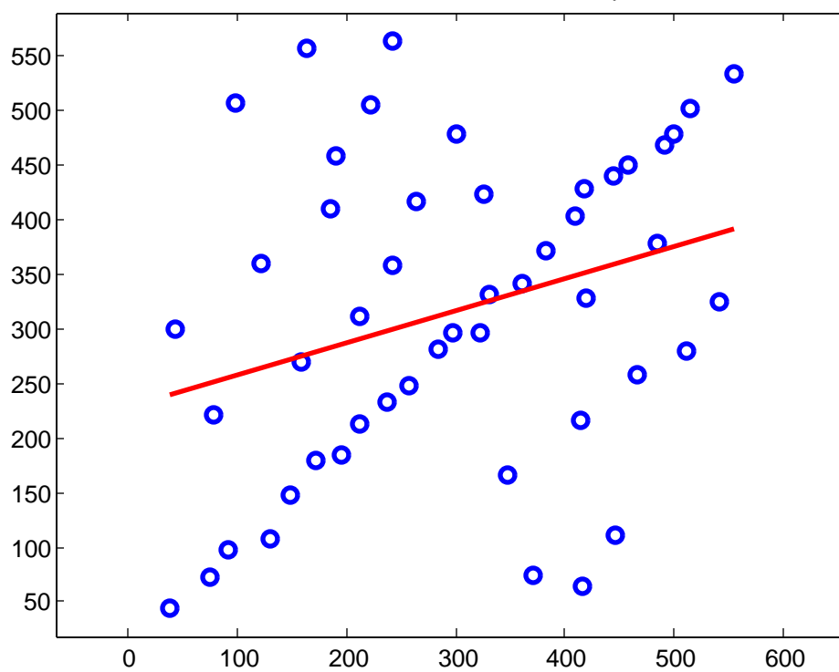
conventional LS fit to all of the data points
