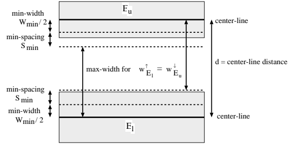
Figure 3. Initialization of upper-bound wire widths.
