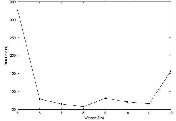
Figure 3. Simulation times for different window sizes.
