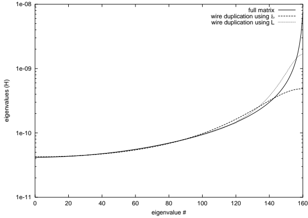
Figure 4. Eigenvalues for full matrix, wire duplication using \mathcal{L} matrix, and wire duplication using L matrix.
