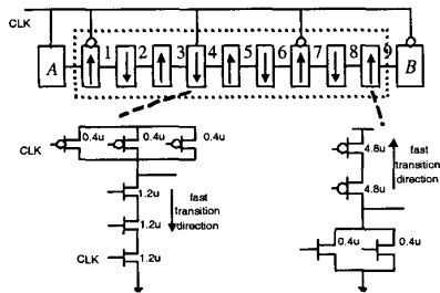
Figure 1: Topology and cascading of skewed logic.
