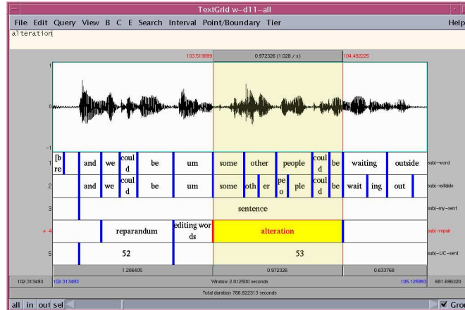
Figure 3. The annotation of a speech repair from the wd11 data set of the KDI visual-audio database.
