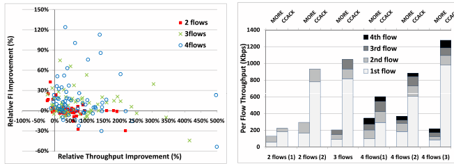
(a) Scatterplot of relative throughput improvement vs. relative FI improvement with 2, 3, and 4 flows. (b) Per-flow throughputs with MORE and CCACK for the 6 scenarios with the largest FI decrease under CCACK.
