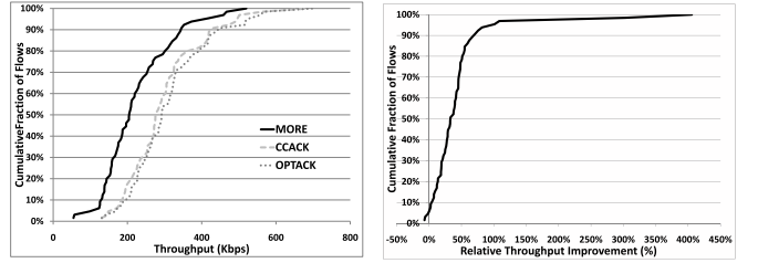
(a) CDF of throughputs achieved with MORE and CCACK. (b) CDF of relative throughput improvement of CCACK over MORE.
