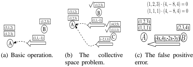
Fig. 3. Null-space-based (NSB) coded feedback.
