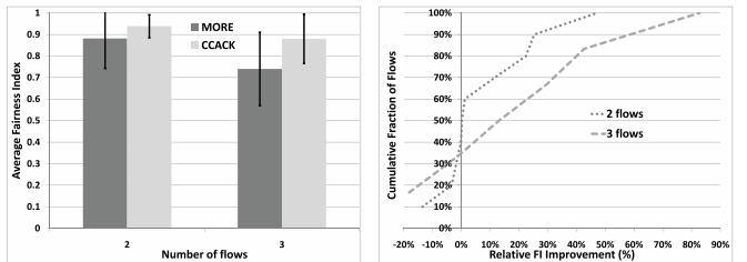
(c) Average per scenario FIs (bars) and standard deviations (lines). (d) CDF of relative FI improvement of CCACK over MORE.
