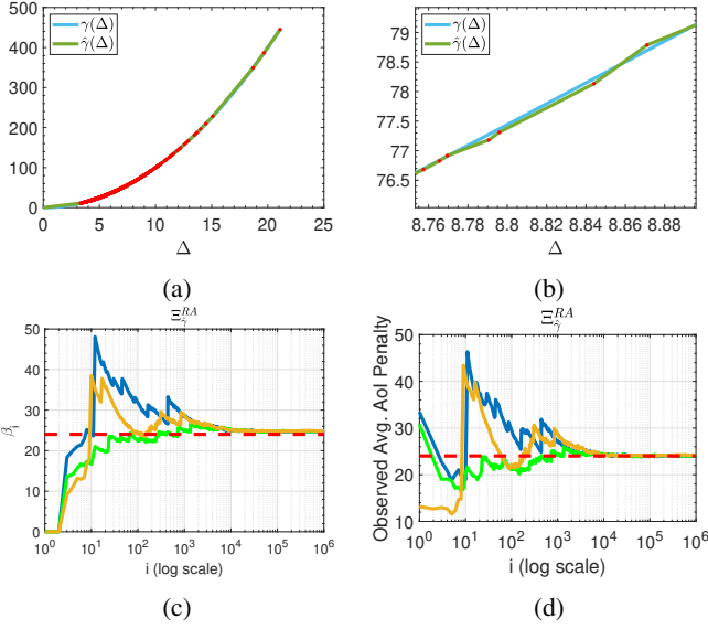
Fig. 6: Simulation results using the online algorithm \Xi_{\hat{\gamma}}^{RA} under the i.i.d. delay.
