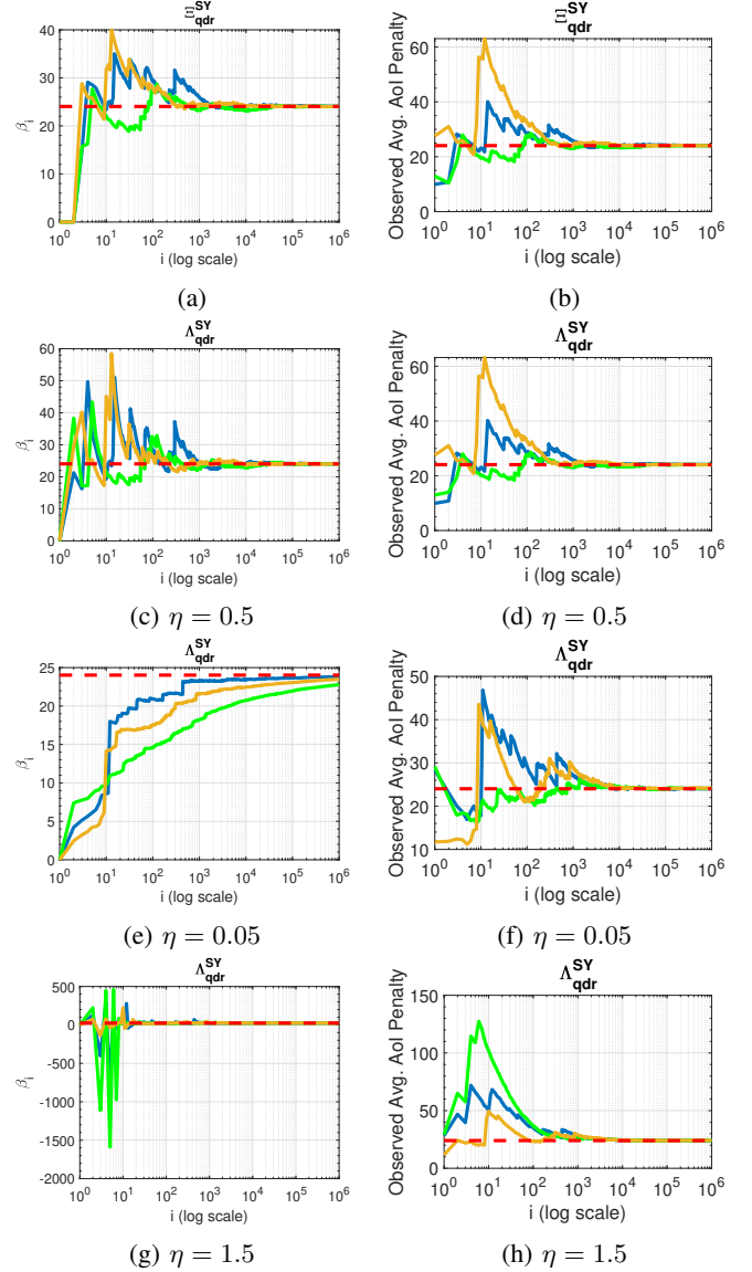
Fig. 4: Left: Evolution of \beta_i using the online algorithms Right: Evolution of the observed AoI penalty using the online algorithms Different curves represent different random seeds. The horizontal red dashed line represents \beta^* .
