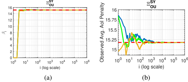
Fig. 10: Simulation results using the bounded \gamma_{\text{OU}}(\cdot) corresponding to the OU process.
