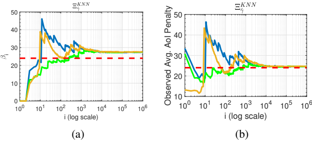
Fig. 7: Simulation results using the online algorithm \Xi_{\hat{\gamma}}^{KNN} under the i.i.d. delay.
