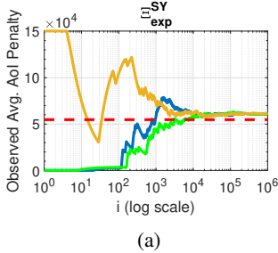
Fig. 8: Simulation results using the online algorithm \Xi_{\hat{\gamma}}^{SY} under the Markov delay.
