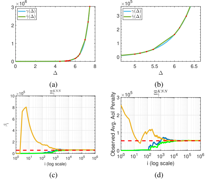
Fig. 9: Simulation results using the online algorithm \Xi_{\hat{\gamma}}^{KNN} under the Markov delay.
