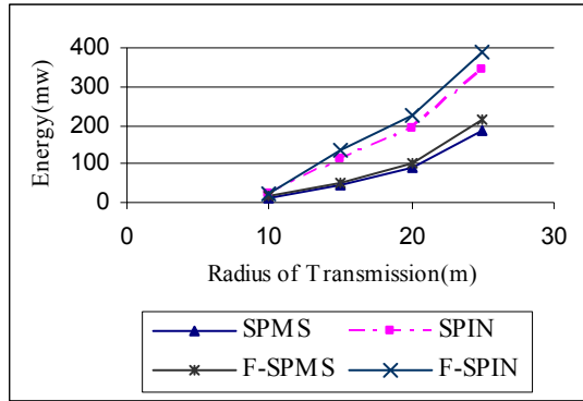
Figure 10: Energy consumed with transmission radius for cluster-based hierarchical communication
