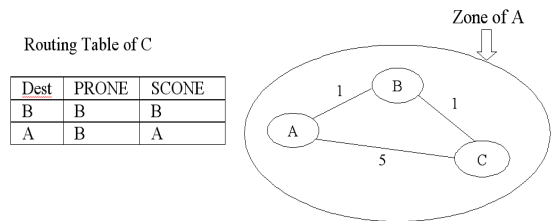
Figure 1. A sample network. Each link has a cost associated with it which represents the transmission power needed to reach the neighbor.
