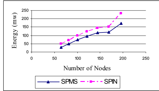
Figure 6: Energy consumed by SPIN and SPMS with varying number of sensor nodes (transmission radius=20 m)
