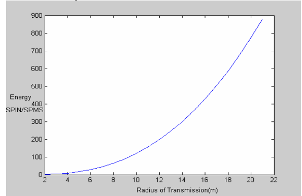
Figure 5. Ratio of Energy (SPIN/SPMS) with varying radius of transmission.
