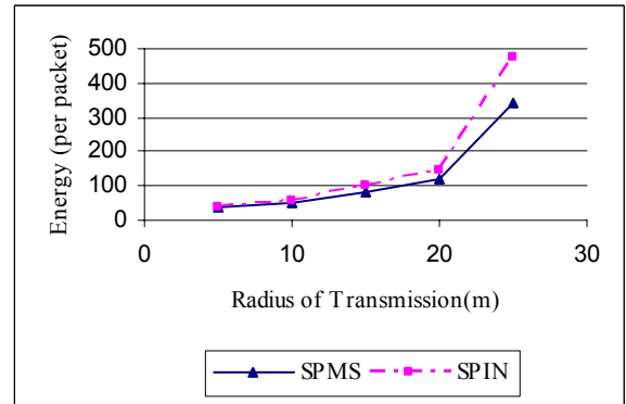
Figure 7: Energy consumed by SPIN and SPMS with different transmission radii (number of nodes=169)
