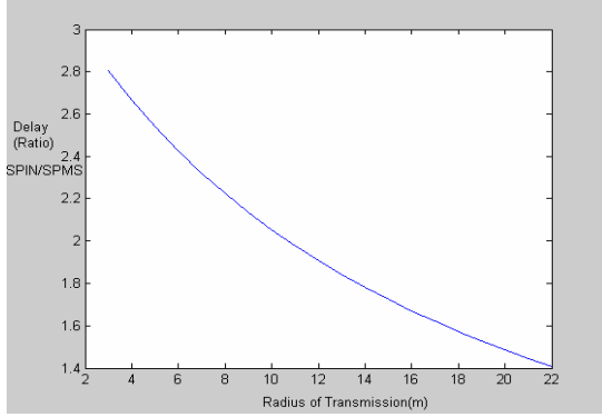
Figure 4. Graph of ratio of end-to-end latency for SPIN to SPMS as the transmission radius varies (obtained from theoretical analysis)
