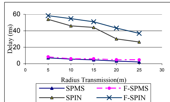
Figure 9: End-to-end delay with transmission radius for static nodes with transient failures.
