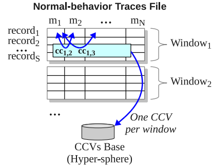
Fig. 4: Creation of the normal-behavior hyper-sphere.
