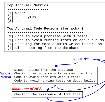
Fig. 11: Results from ORION for the MHM problem.
