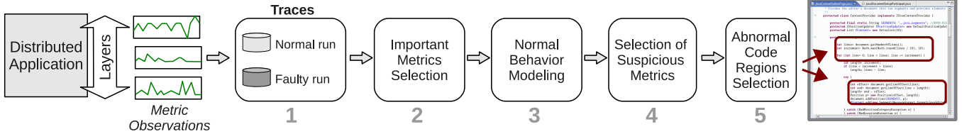
Fig. 2: Overview of the problem determination workflow.
