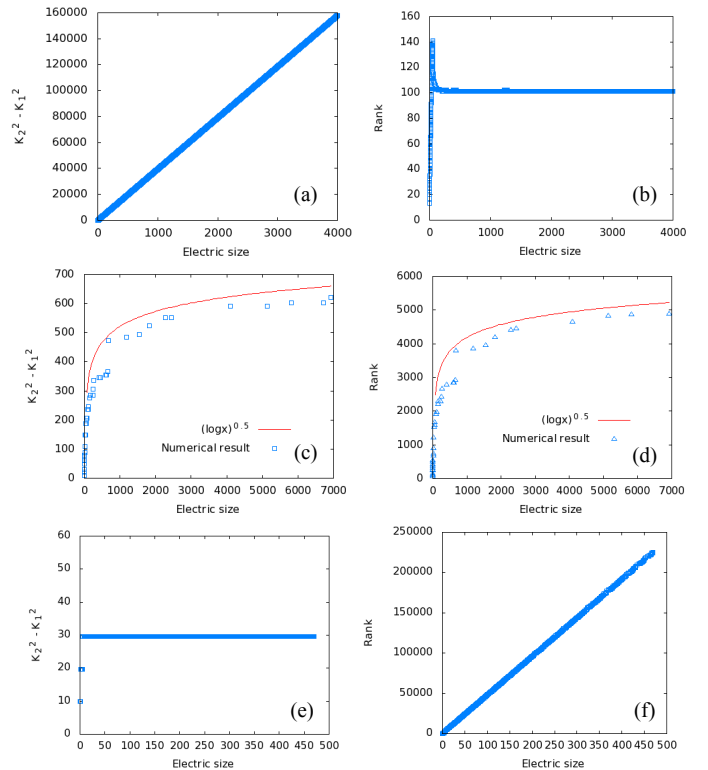
Figure. 1. The upper bound of \Delta_{\min} ( K_2^2 - K_1^2 ) and rank k with respect to electric size. (a-b) 1-D problems; (c-d) 2-D problems; (e-f) 3-D problems.
