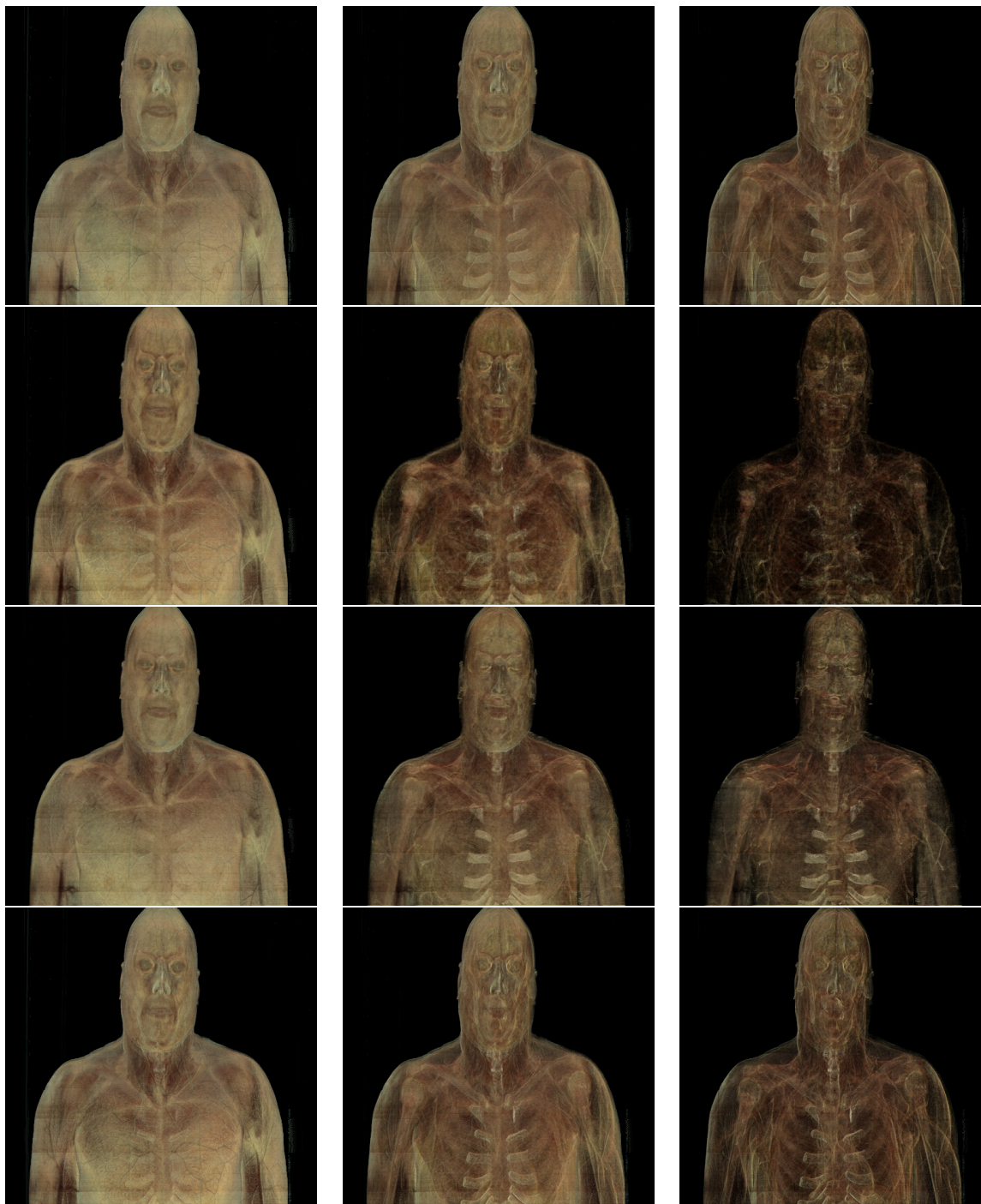
Figure 5: Renderings of the upper torso region using the L^* component. From top to bottom: First Row) Equation (1): Color distance gradient magnitude function. Second Row) Equation (9): Gradient dot product function. Third Row) Equation (7): Second directional derivative "only" function. Fourth Row) Equation (8). First and second directional derivative function. From left to right: Left) k_{gc}=0.0 , k_{gs}=0.75 , k_{ge}=0.5 . Center) k_{gc}=0.0 , k_{gs}=0.75 , k_{ge}=1.0 . Right) k_{gc}=0.0 , k_{gs}=0.75 , k_{ge}=1.5 <see color section>.
