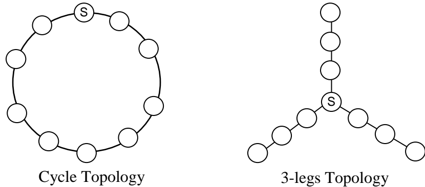
Figure 24: Illustration of the two topologies in the SYSADMIN domain (10 nodes). Each node represents a machine. The “S” label indicates a server machine, as specified in the work of Patrascu et al. (2002).
