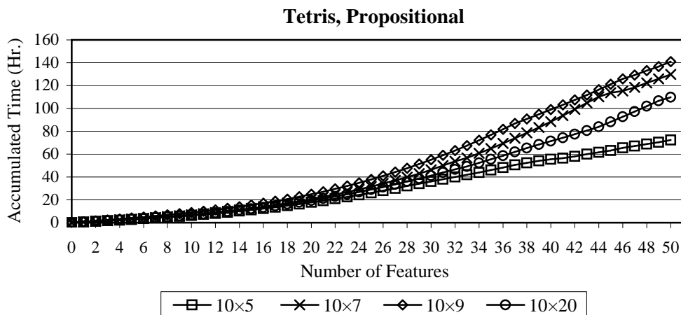
Figure 8: Plot of the accumulated time required to reach each point in Figure 7, averaged over two trials.
