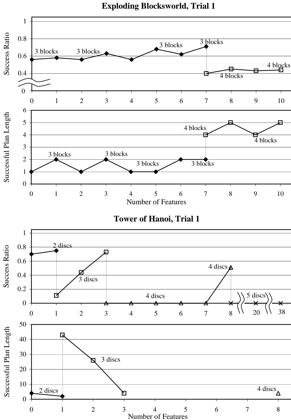
Figure 19: Summary results for EXPLODING BLOCKSWORLD and TOWERS OF HANOI. For full discussion and detailed results, please see Appendix B.
