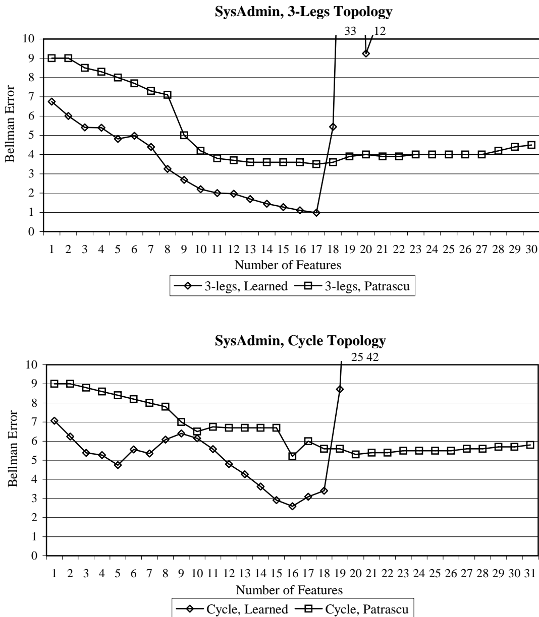
Figure 25: L_\infty Bellman error for the SYSADMIN domain (10 nodes) for two topologies. Values for the results from the work of Patrascu et al. (2002) are taken from Figure 2 and 3 of the work of Patrascu et al. (2002).
