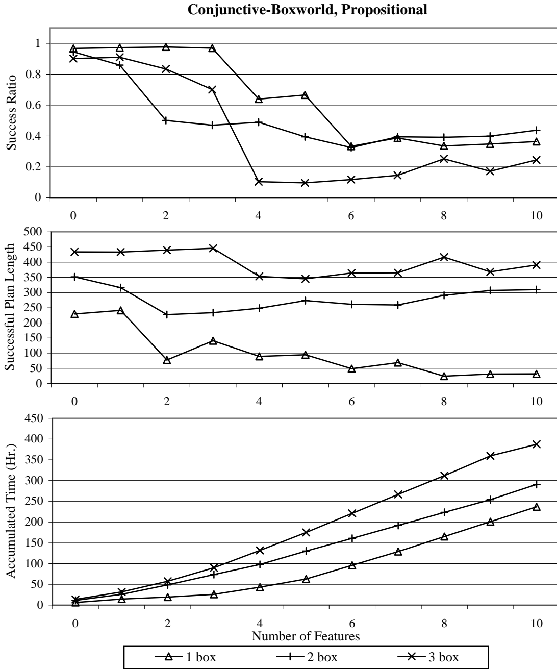
Figure 17: CONJUNCTIVE-BOXWORLD performance (averaged over 600 problems) and accumulated run-time for propositional learner, averaged over two trials. Throughout the learning process the number of cities is 5.
