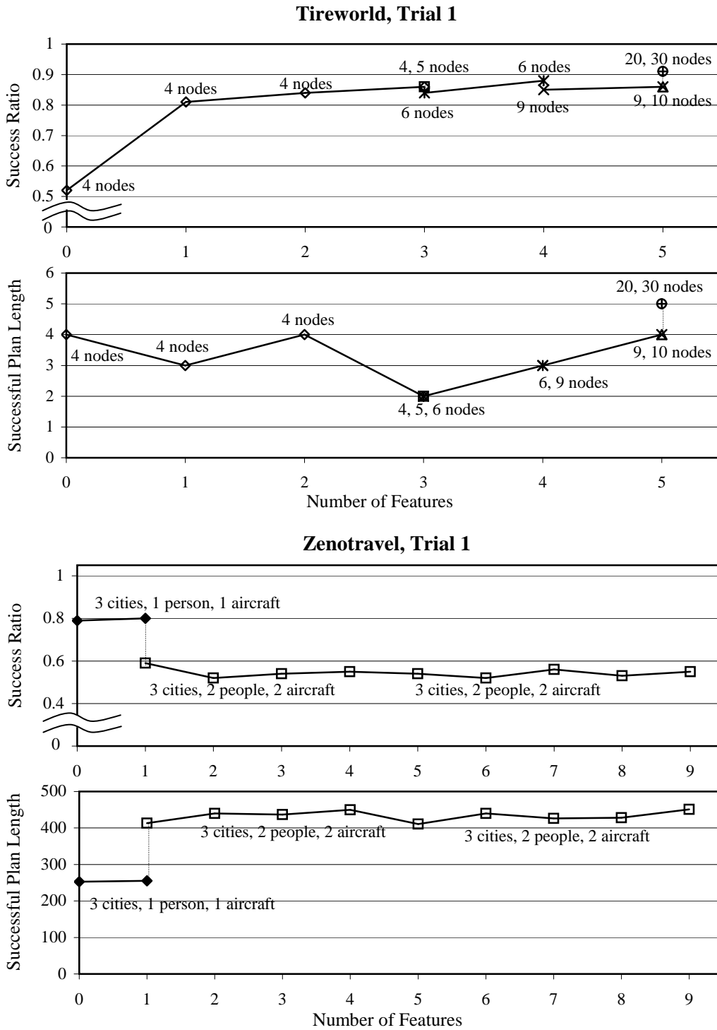
Figure 18: Summary results for TIREWORLD and ZENOTRAVEL. For full discussion and detailed results, please see Appendix B.
