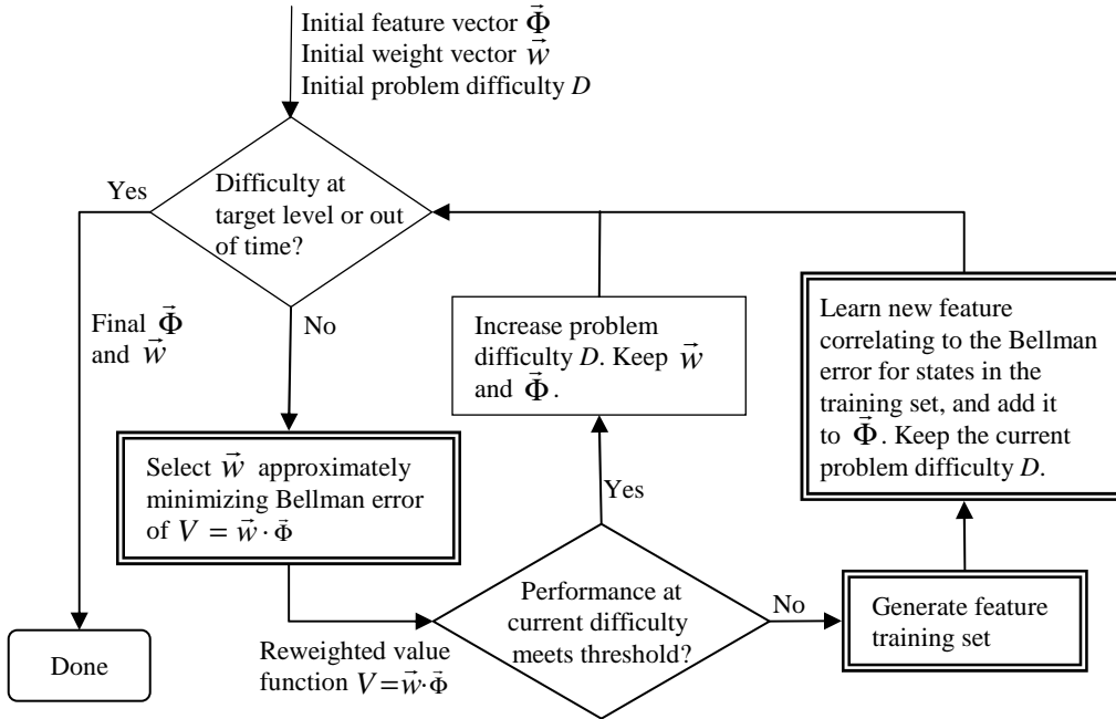
Figure 1: Control flow for feature learning. Boxes with double borders represent assumed subroutines for our method. We assume that the problem distribution is parameterized by problem difficulty (such as problem size).
