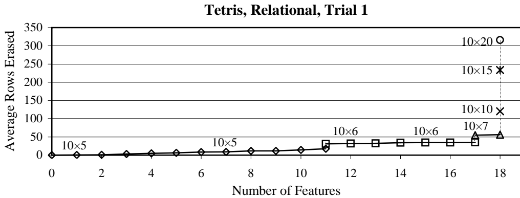
Figure 6: Plot of the average number of lines erased over 10,000 TETRIS games after each run of AVI training during the learning of relational features (trial 1). Vertical lines indicate difficulty increases (in the number of rows), as labeled along the plot.
