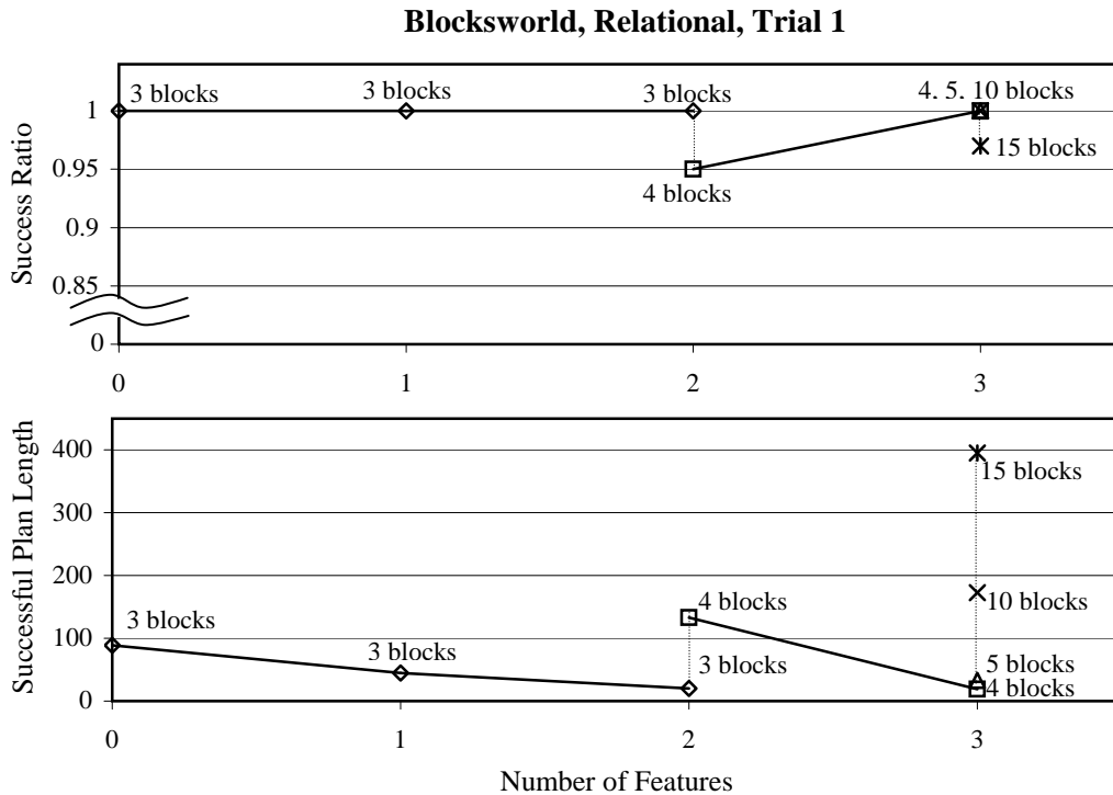
Figure 13: BLOCKSWORLD success ratio and average successful plan length (averaged over 600 problems) for the first trial from Figure 12 using our relational learner.
