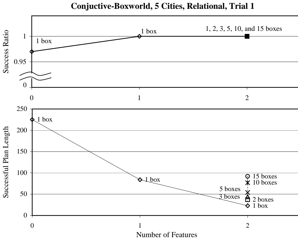
Figure 16: CONJUNCTIVE-BOXWORLD success ratio and average successful plan length (averaged over 600 problems) for the first trial using our relational learner.
