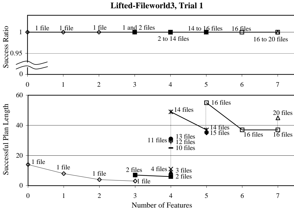
Figure 20: Summary results for LIFTED-FILEWORLD3. For full discussion and detailed results, please see Appendix B.
