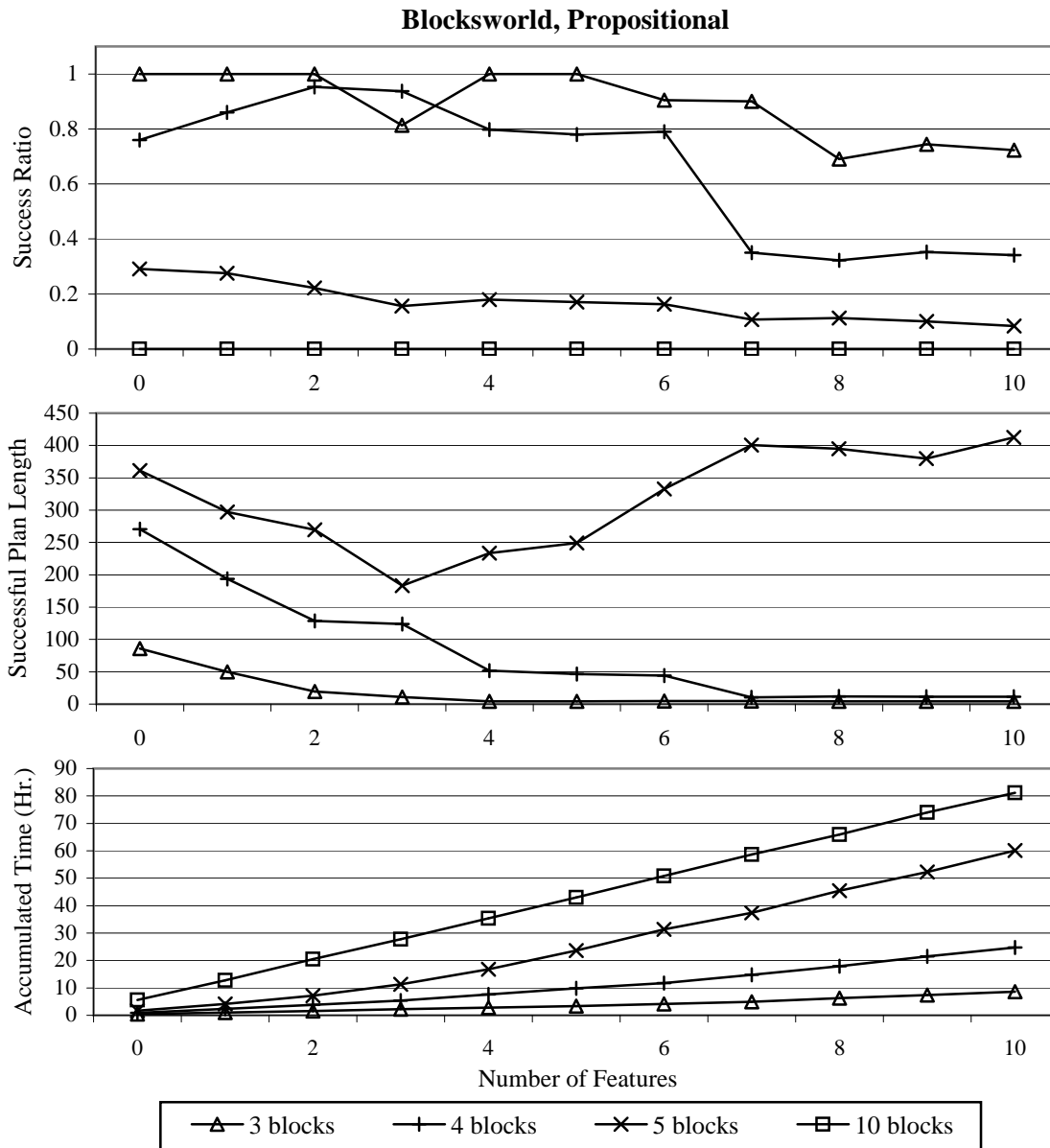
Figure 14: BLOCKSWORLD performance success ratio and average successful plan length (averaged over 600 problems), and accumulated run-time for our propositional learner, averaged over two trials.
