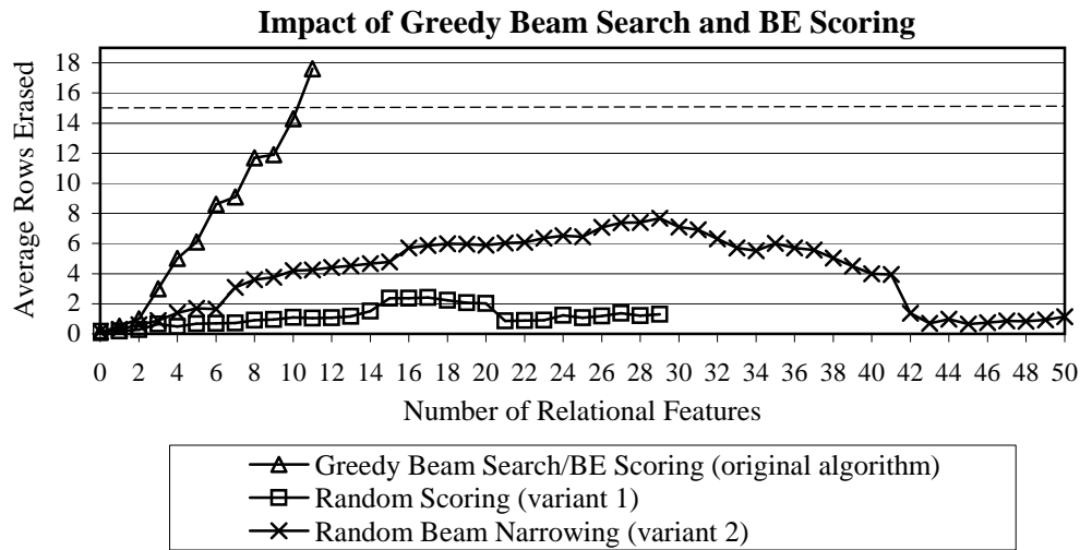
Figure 9: Plot of the average number of lines erased in 10,000 TETRIS games for relational features learned from the original algorithm and the two alternatives as discussed in Section 6.2. For Random Scoring and Random Beam Narrowing, the results are averages over two independent trials. Trials of these two variants are terminated when they fail to make progress for several feature additions. For comparison purposes, trial one of the original Greedy Beam Search/BE Scoring method is shown, reaching the threshold for difficulty increase after eleven feature additions (trial two did even better).
