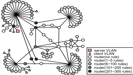
Figure 10: Layer-3 topology showing systematic distribution of ACL rules after applying fine-grained, LB placement strategy.
