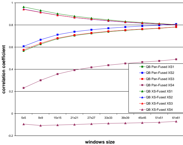
Figure 3. Effect of different window sizes on correlation coefficients
