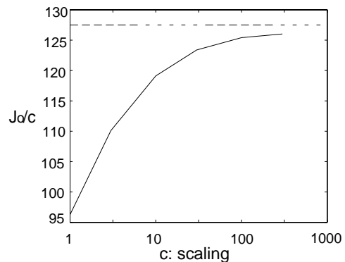
Fig. 4. The static pricing policy compared with the upper bound: when the capacity of link 3 is 5 bandwidth units and the service time distribution is Pareto.
